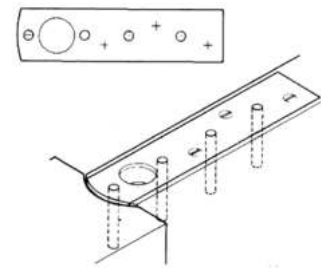
Pivot Mechanism
